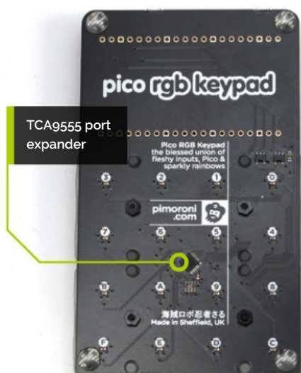
▲ Figure 4 The TCA9555 port expander is the small square integrated circuit mounted on the rear of the keypad PCB
