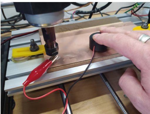
Figure 8 ◆ Using the Z probe upside down to zero the tool directly onto the PCB board
